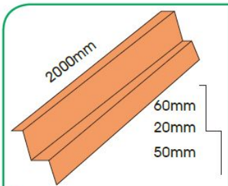
Wall Side Flashing
