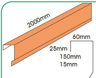
Barge Board Cover
